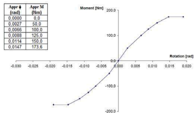
Momentstyvhet i horisontalled, M_{z,d}
